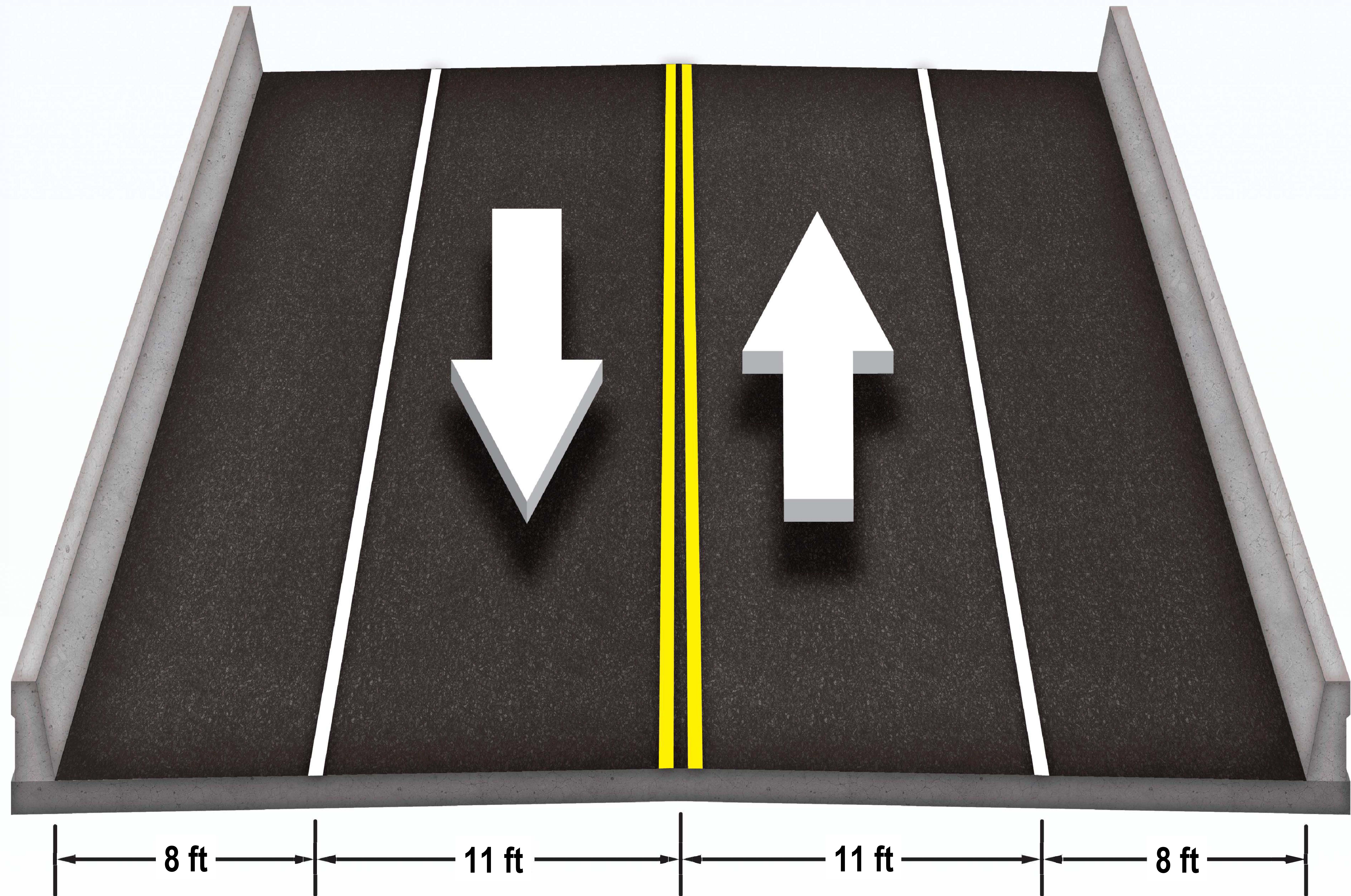
Proposed Bridge Typical Section CR 361B over Rocky Creek Bridge Replacement
